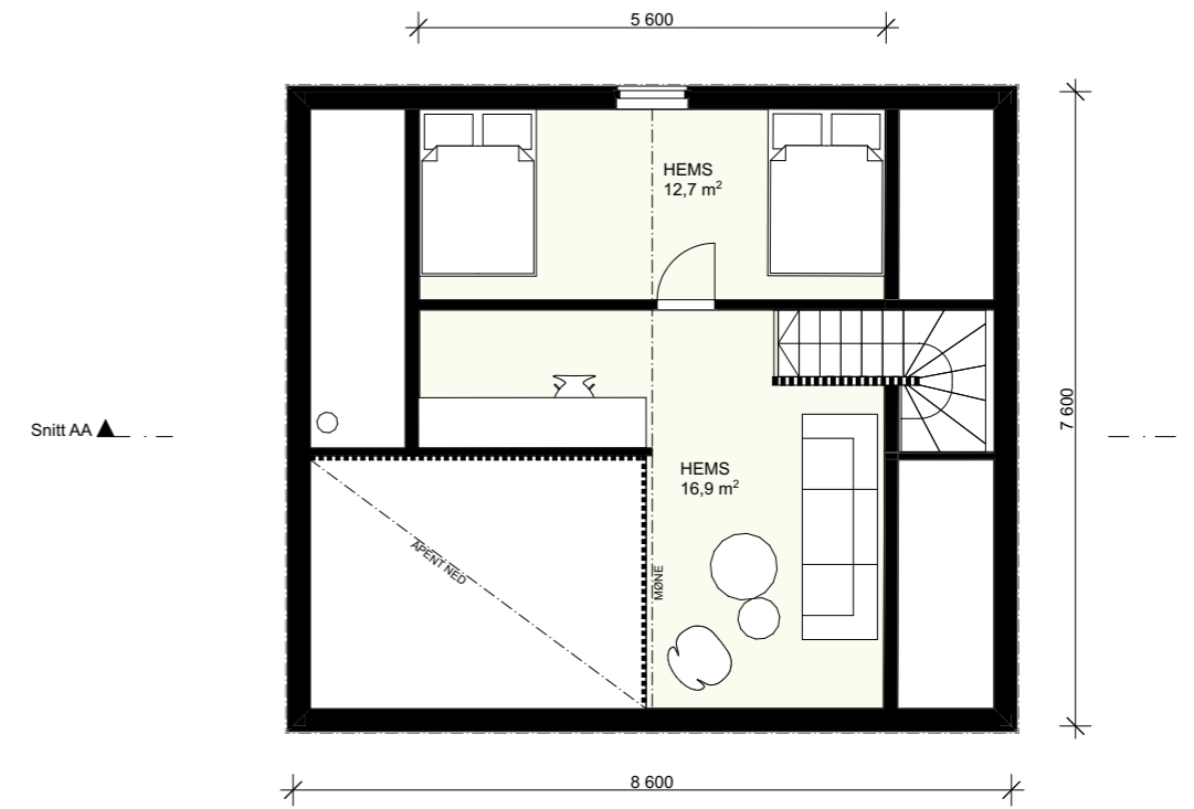
PLAN HEMS
