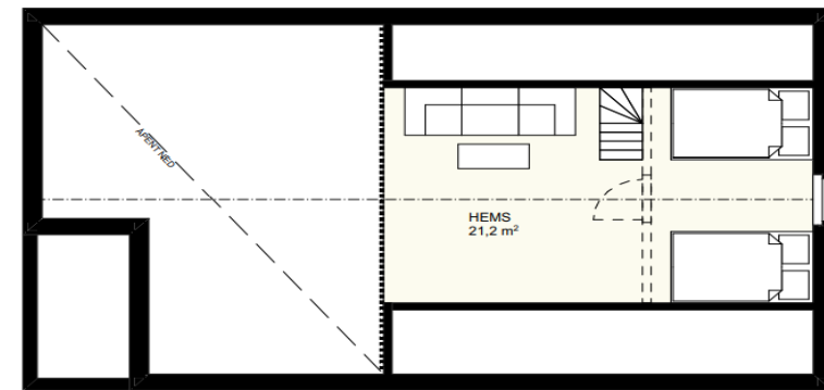
PLAN HEMS
