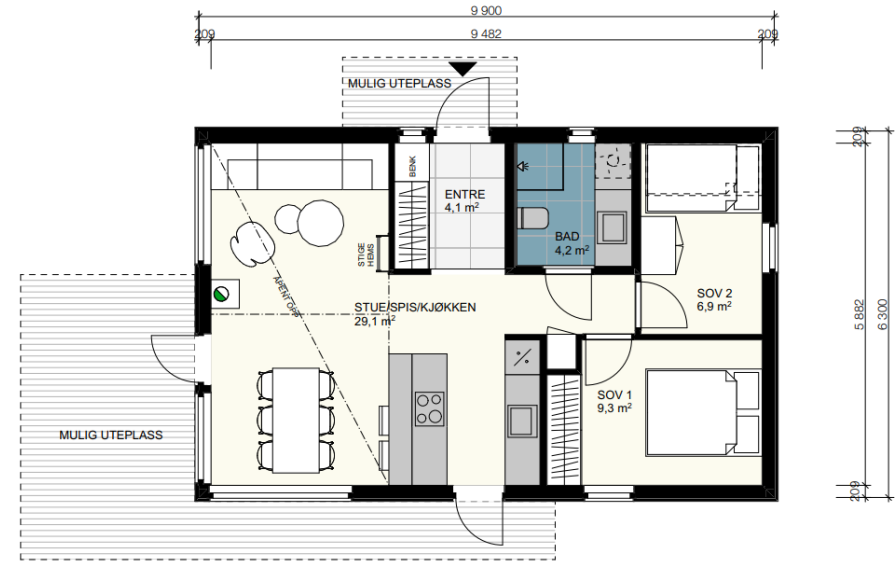
PLAN 1
