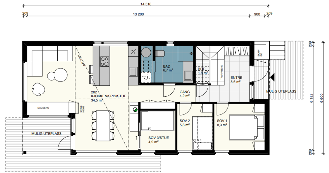
PLAN 1
