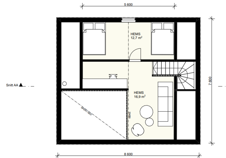
PLAN HEMS
